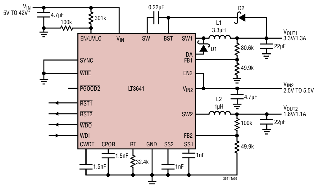
2MHz 3.3V/1.3A and 1.8V/1A Buck Regulators
